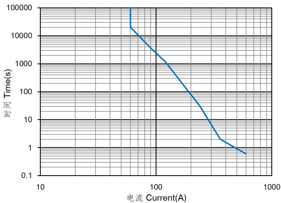
电流承载曲线 Current Carry Curve:
